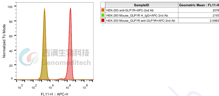
Figure 1 | Mouse_GLP1R HEK-293 Cell Line was determined by flow cytometry using Anti-H_GLP1R hIgG1 Antibody(glutazumab) (Genomeditech/GM-84914AB).
